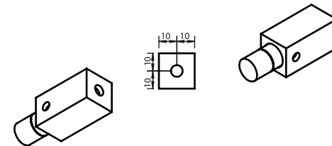
Bracket Assembly
